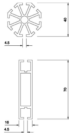
Post and Beam section sizes (mm)
